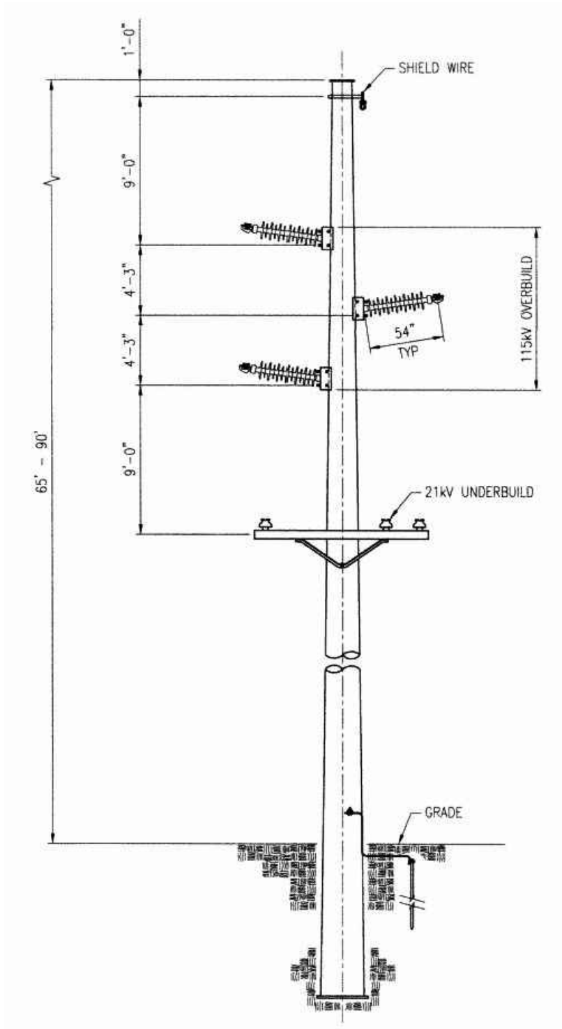
Figure 9 Single Pole Structure With 115kV Overbuild
